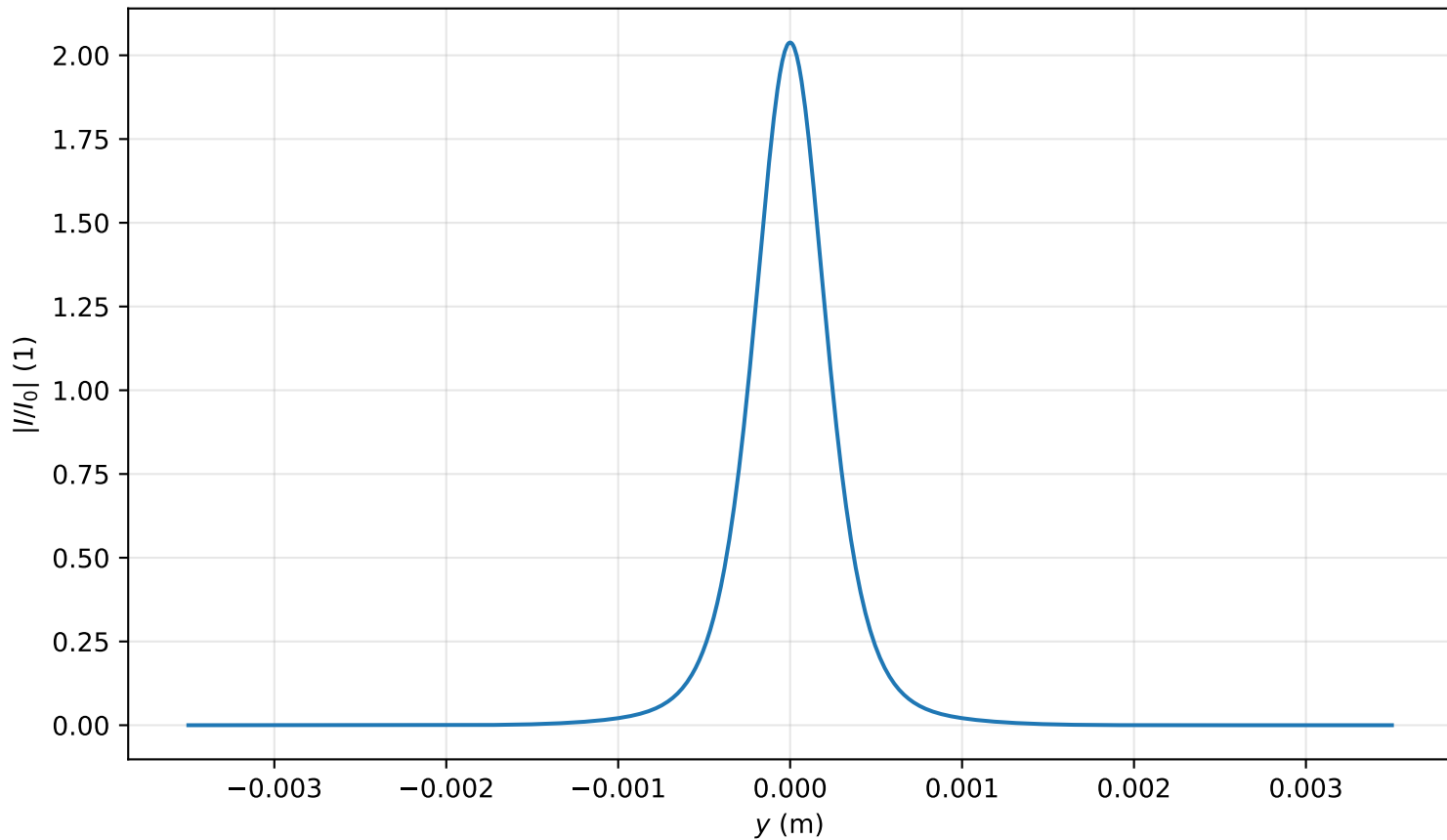
Intensity profile I(x=0, y, z=1.831)/I_0 , P_{in}=1.0P_{cr} , artificial time
